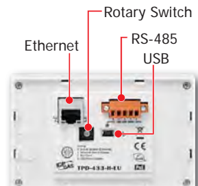
TPD-433-H-EU Rear View
