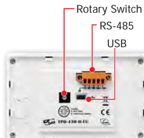
TPD-430-H-EU Rear View
