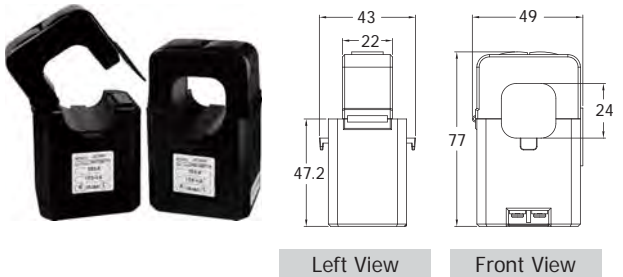
240: CTΦ24mm (200 A Max.)
