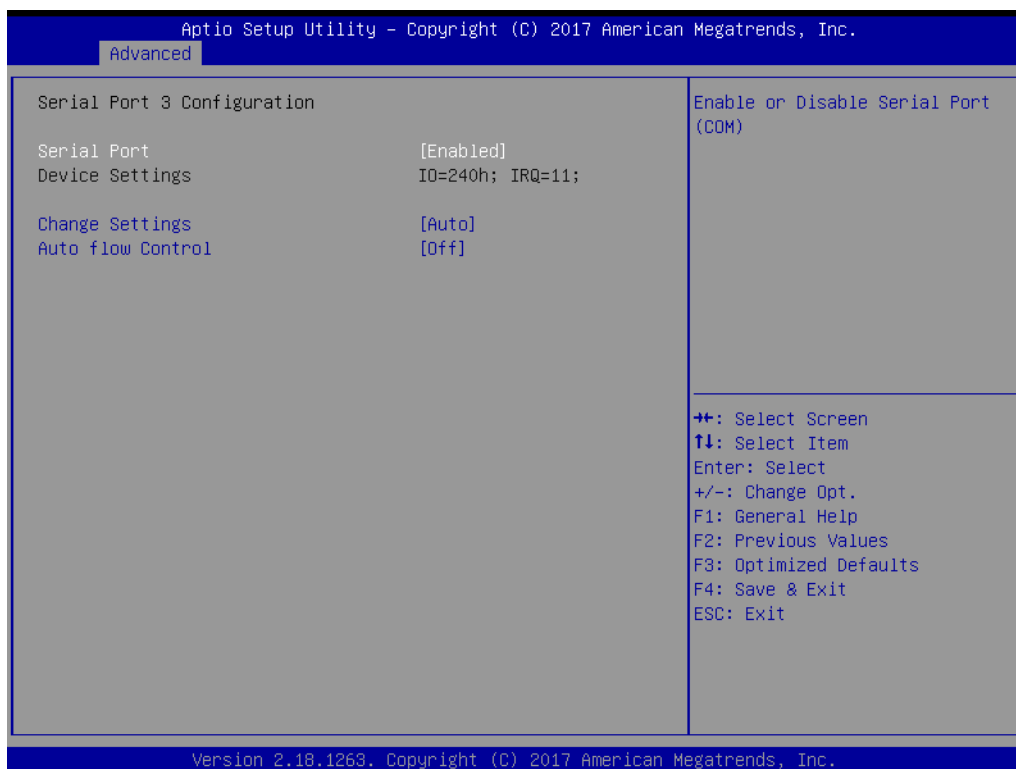
Figure 3.15 Serial Port 3 Configuration
