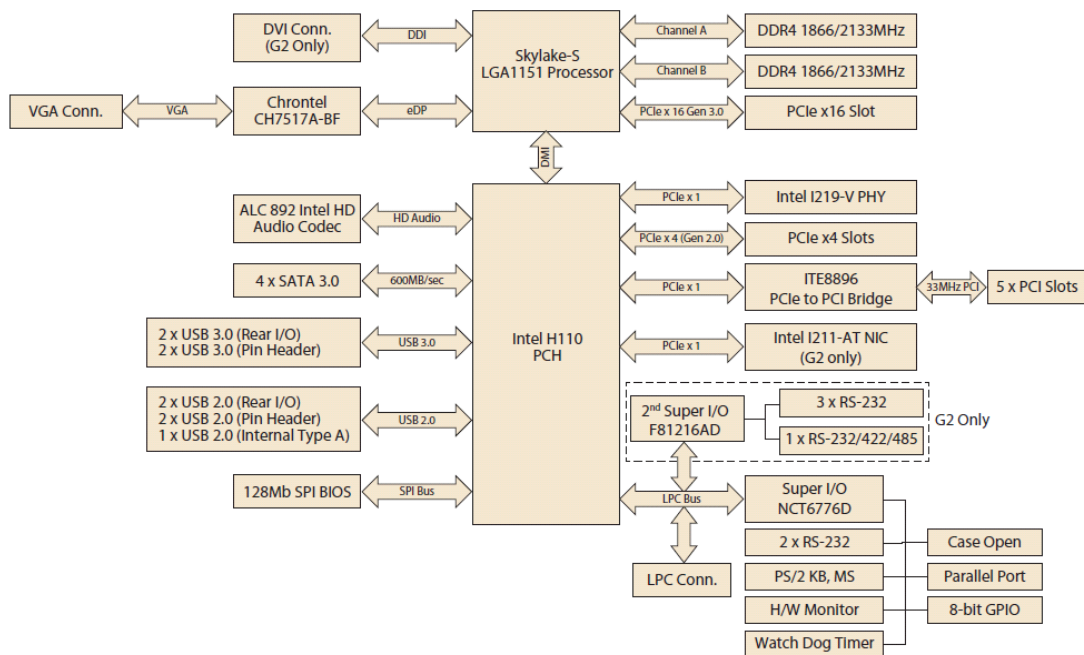
Figure 1.3 AIMB-705 Block Diagram
