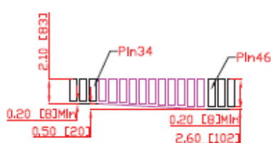
Detail C 30µ gold finger
