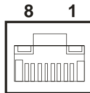
Figure 2.16 Ethernet Connector
