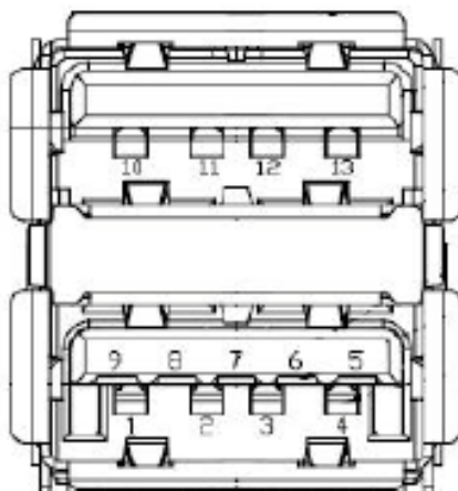
Figure 2.18 USB Connector
