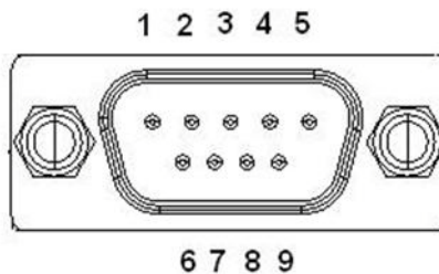
Figure 2.27 COM Port Connector
