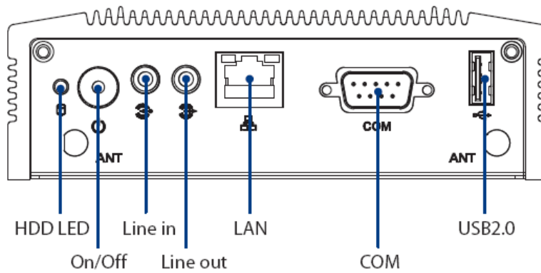
Figure 2.3 ARK-1123C front view
