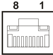
Figure 2.9 Ethernet Connector
