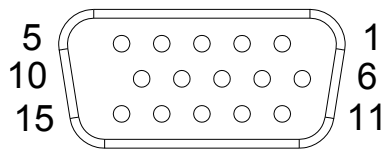
Figure 2.17 VGA Connector
