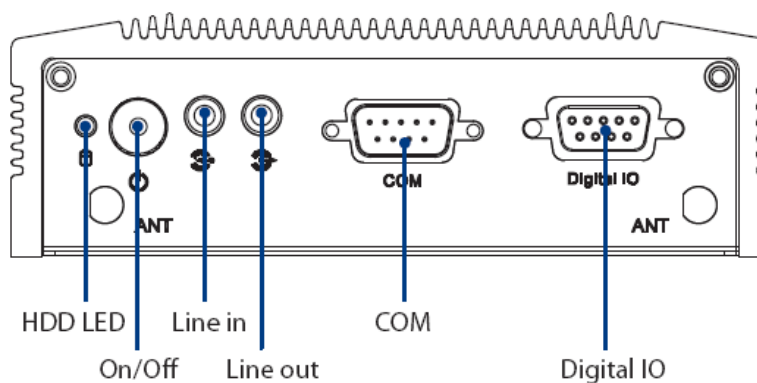
Figure 2.5 ARK-1123C front view
