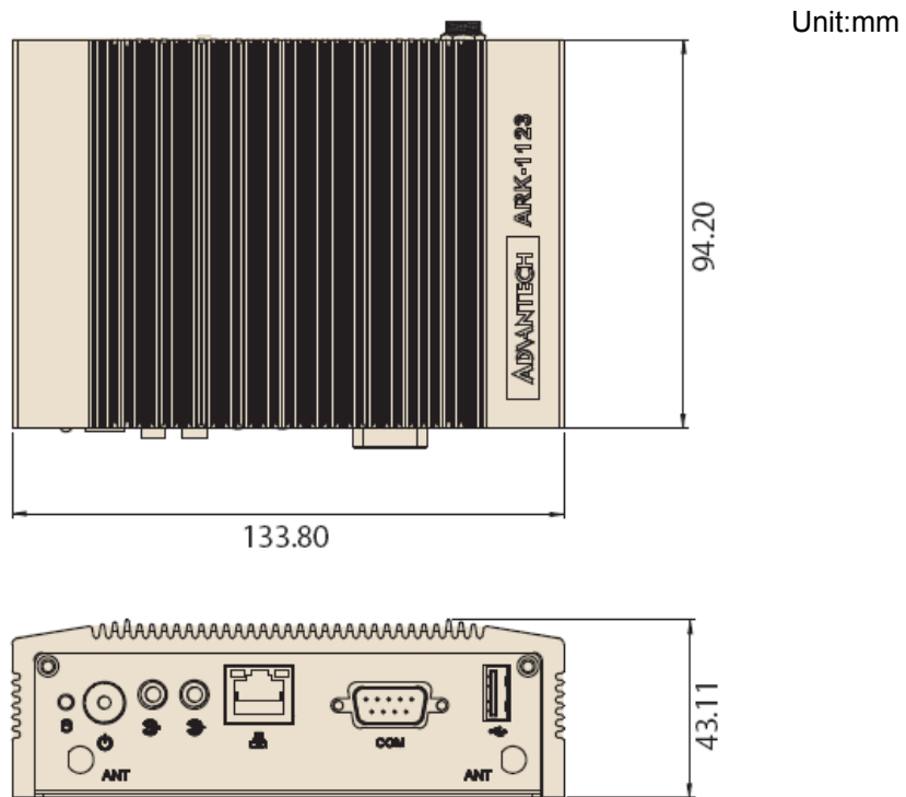
Figure 1.3 ARK-1123L mechanical dimension drawing
