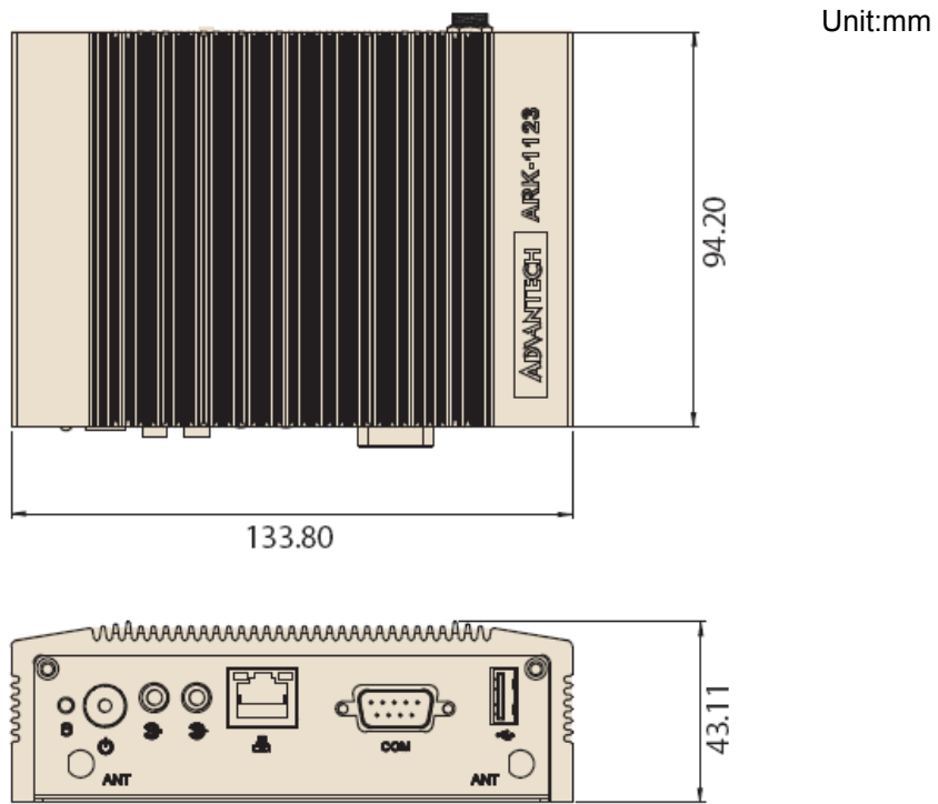
Figure 1.2 ARK-1123C mechanical dimension drawing
