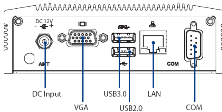
Figure 2.4 ARK-1123C rear view
