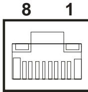
Figure 2.23 Ethernet Connector
