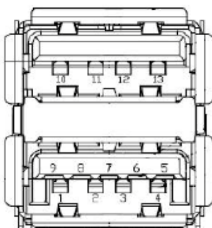
Figure 2.25 USB Connector
