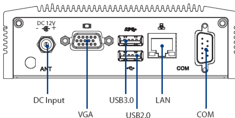
Figure 2.6 ARK-1123C rear view
