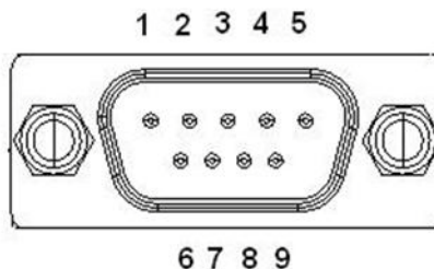
Figure 2.20 COM Port Connector
