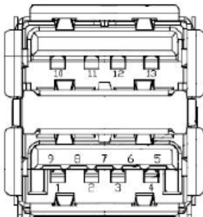
Figure 2.10 USB Connector
