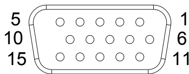
Figure 2.24 VGA Connector
