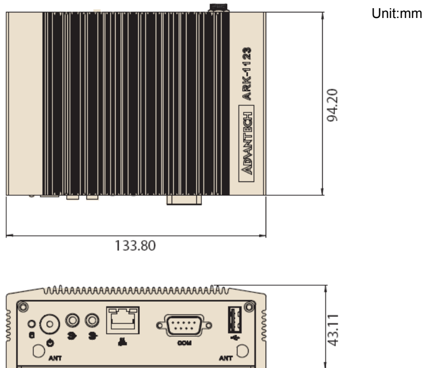
Figure 1.1 ARK-1123H mechanical dimension drawing
