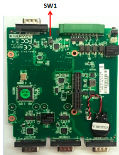
Figure 3.2 Top side of I/O board
