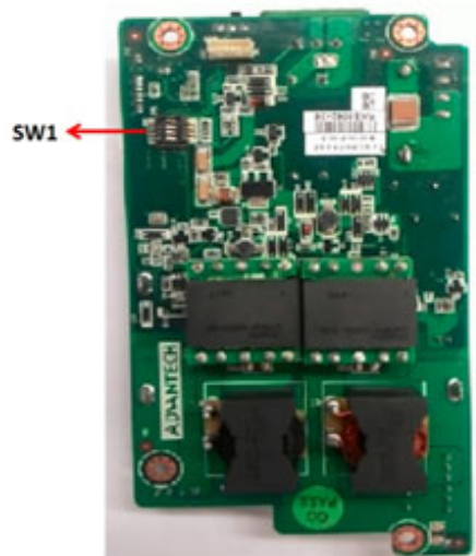
Figure 3.5 Top side of power board
