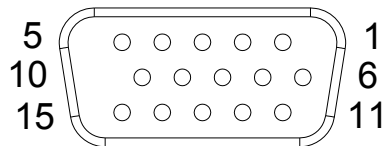
Figure 4.1 VGA Connector
