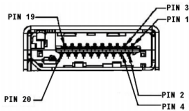
Figure 4.17 HDMI Connector
