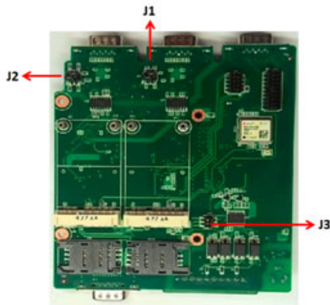
Figure 3.3 Bottom side of I/O board
