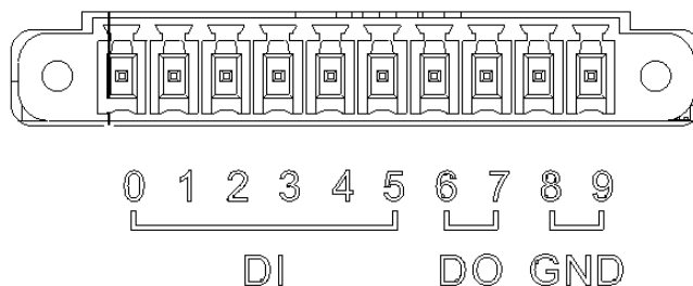
Figure 4.18 DIO Connector
