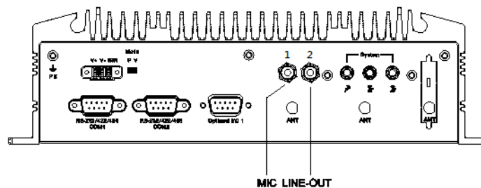
Figure 4.9 Cellular Voice Connector
