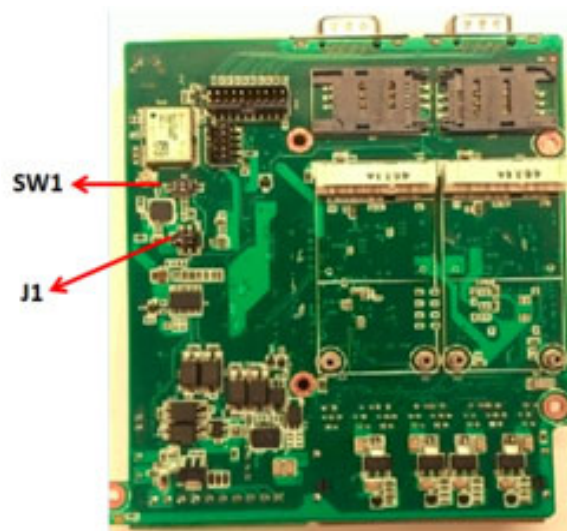
Figure 3.4 Bottom side of I/O board
