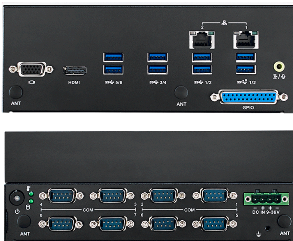
Figure 2.2 ARK-3531 Front and Rear I/O Connector Diagram
