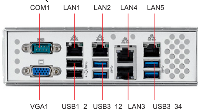
Figure 1.2 Rear I/O of full SKU (ASMB-815T2-00A1E)
