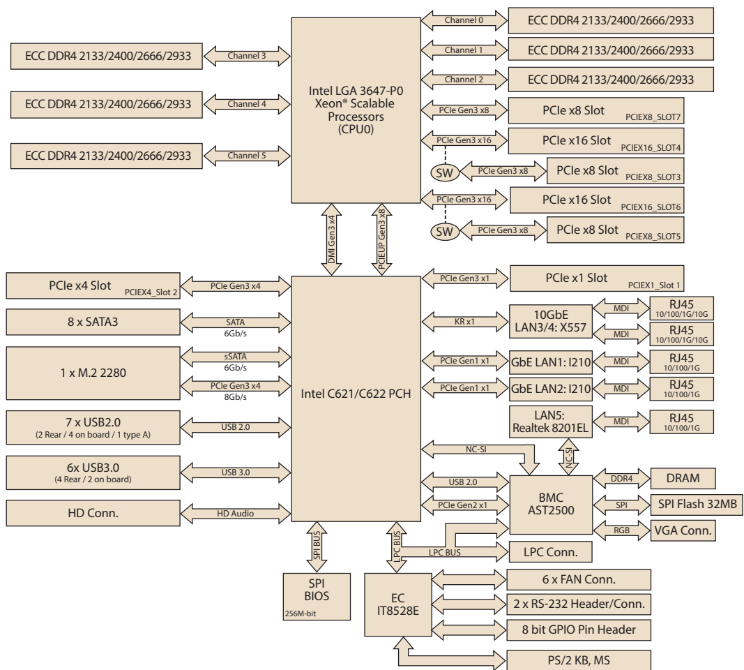
Figure 1.3 Block Diagram
