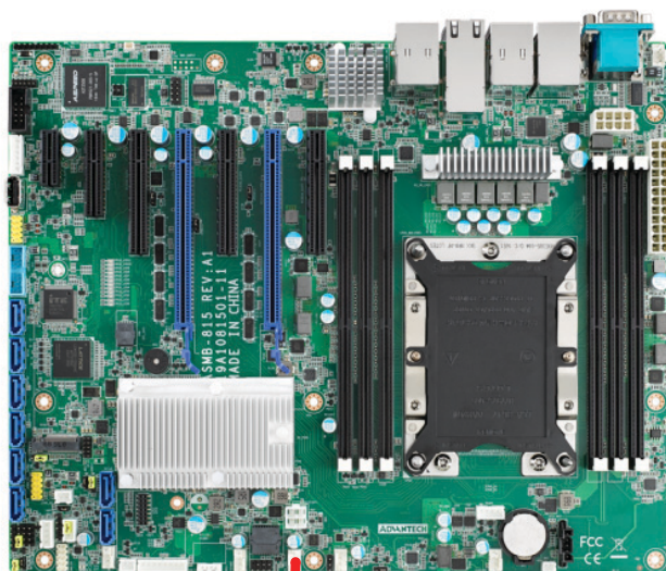
CPU FAN0
