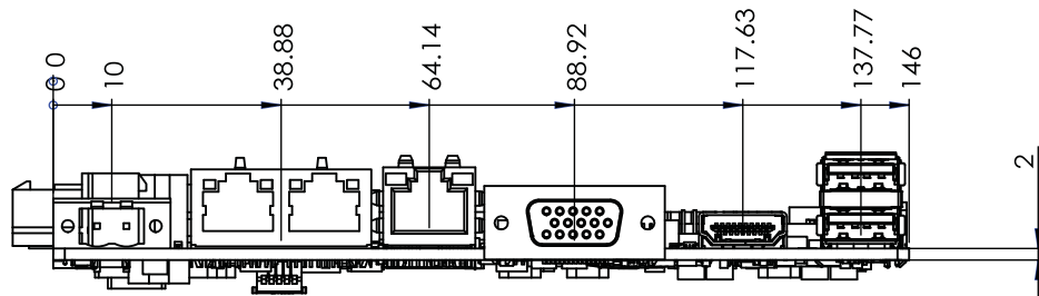
Figure 1.3 MIO-5850 Mechanical Drawing (Coastline)
