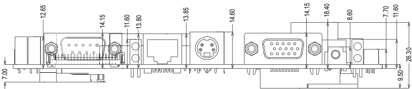
Figure C.3: Dimension of PCM-9375 for H
