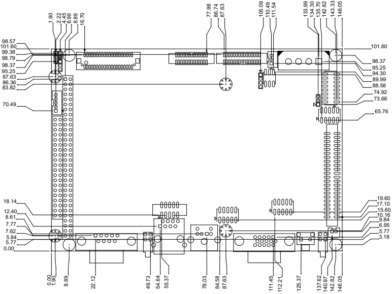
Figure C.1: Dimension of PCM-9375F (TTL)
