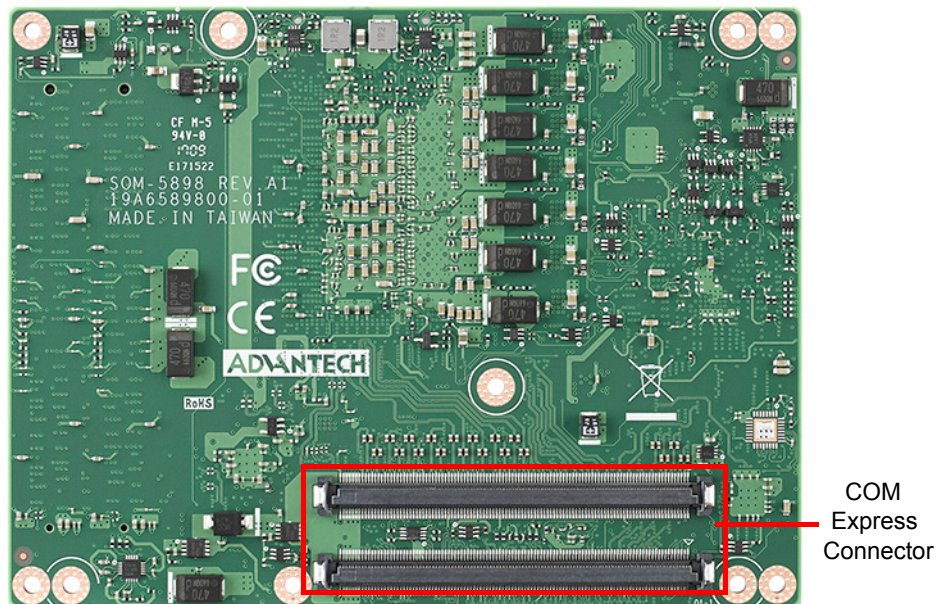
Figure 2.2 Board chips identify – Rear
