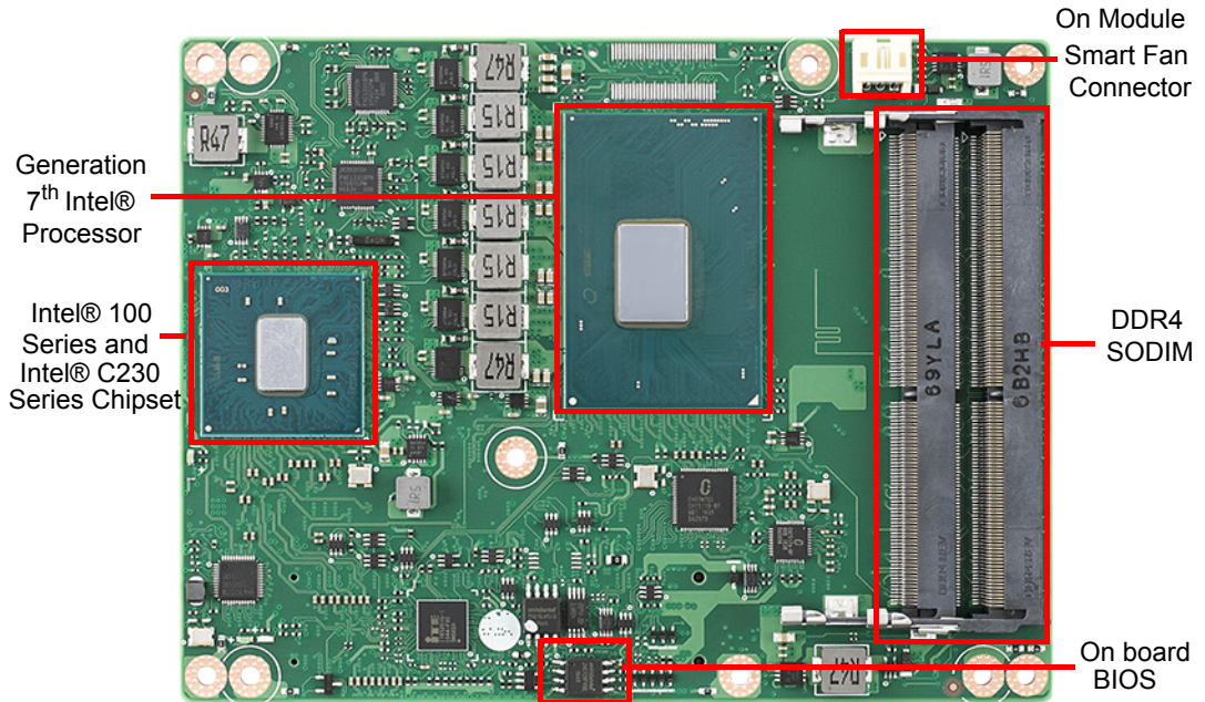
Figure 2.1 Board chips identify – Front
