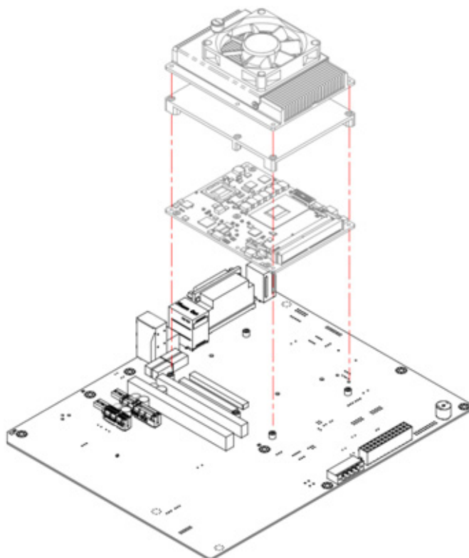
Figure 2.6 Assembly Drawing
