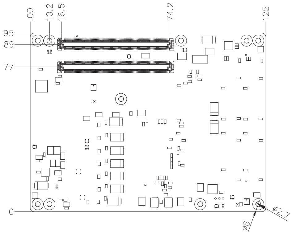
Figure 2.4 Board Mechanical Drawing – Rear
