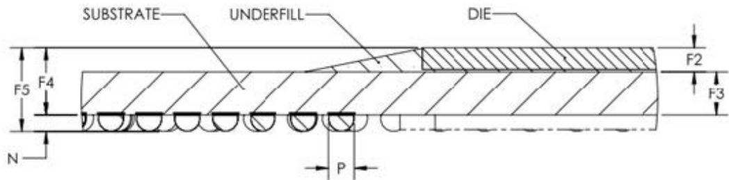
Figure 2.7 CPU 4C+2 Height and Tolerance
