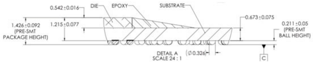
Figure 2.8 PCH Height and Tolerance
