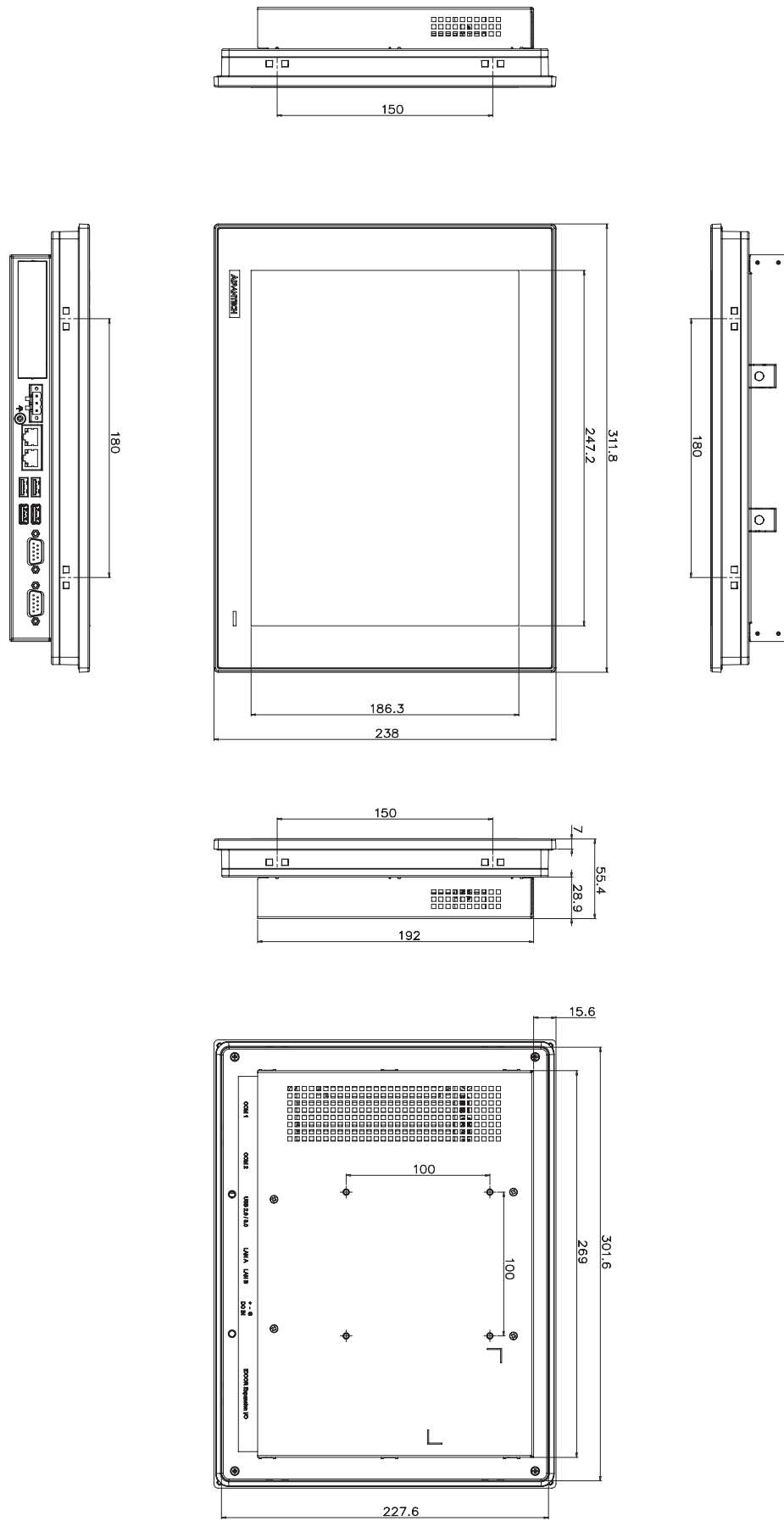
Figure 1.3 TPC-1251T Dimensions
