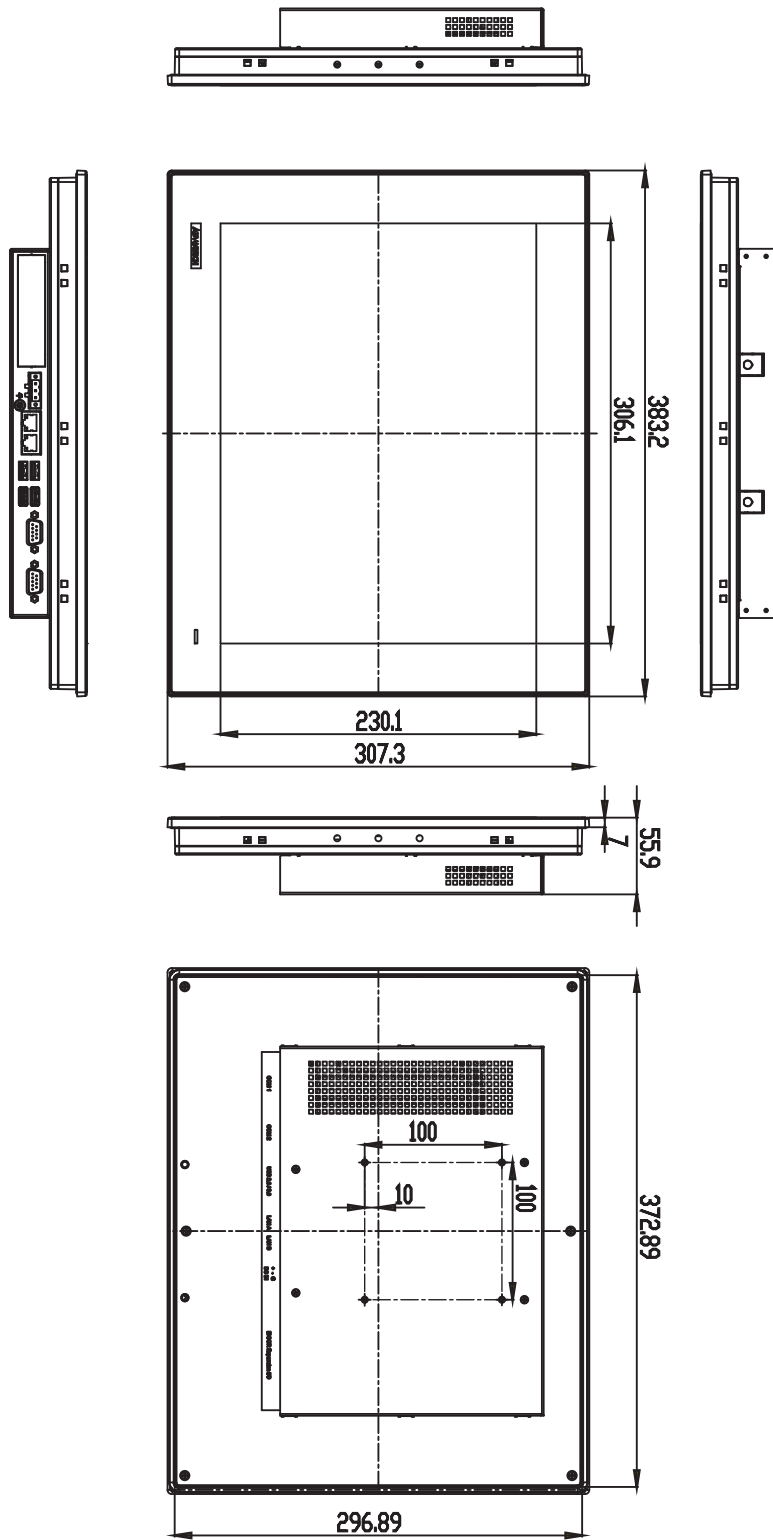
Figure 1.2 TPC-1551T Dimensions
