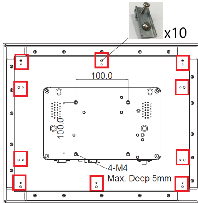
▲ P6151-V3 Panel Mount kits
