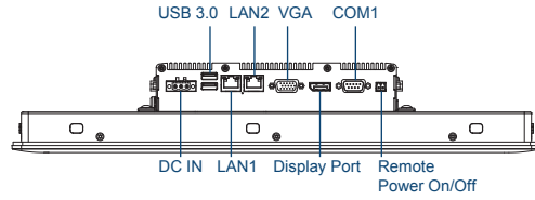
Rear I/O
