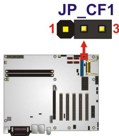
Figure 4-12: LCD Voltage Selection Jumper Location
