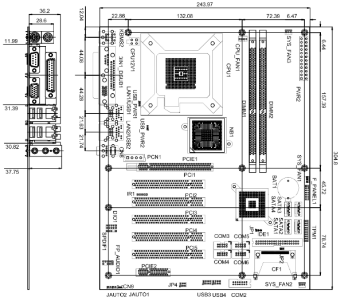
Figure 1-3: Dimensions (mm)
