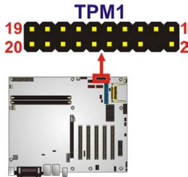
Figure 3-19: TPM Connector Pinout Location
