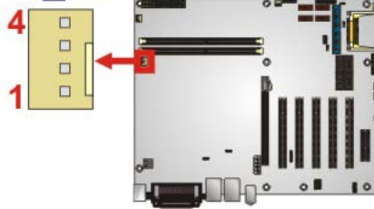
Figure 3-3: CPU Fan Connector Location
