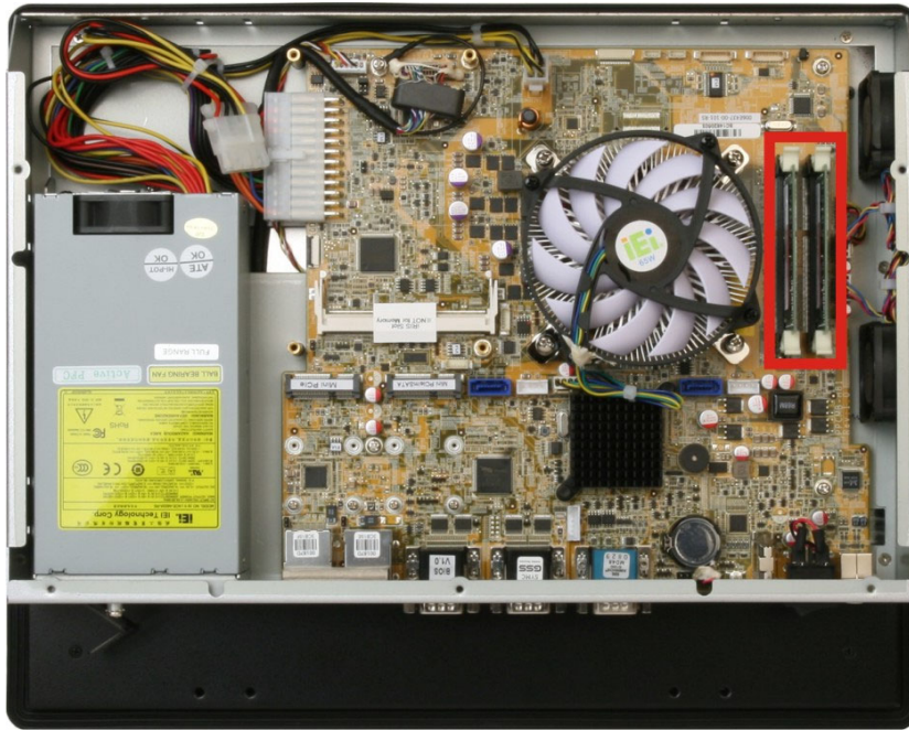
Figure 4-1: SO-DIMM Module Locations
