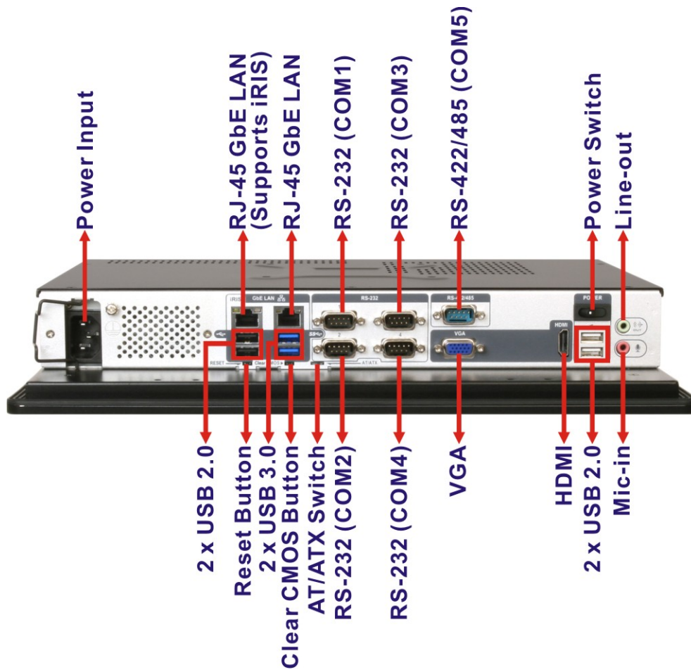
Figure 1-4: Bottom View
