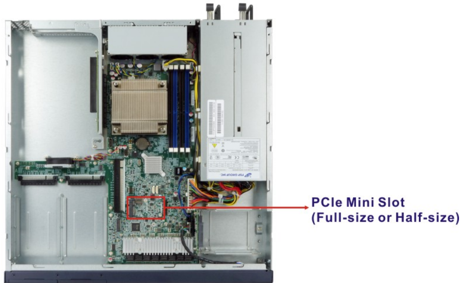
Figure 3-13: PCIe Mini Slot Location
