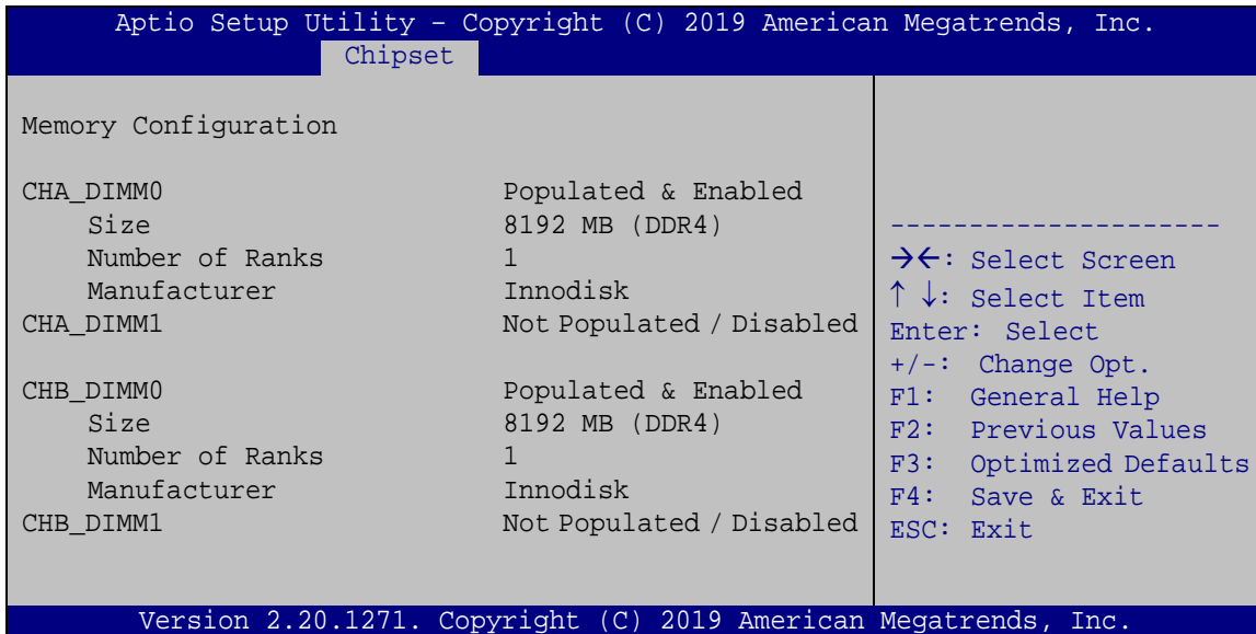
BIOS Menu 14: Memory Configuration
