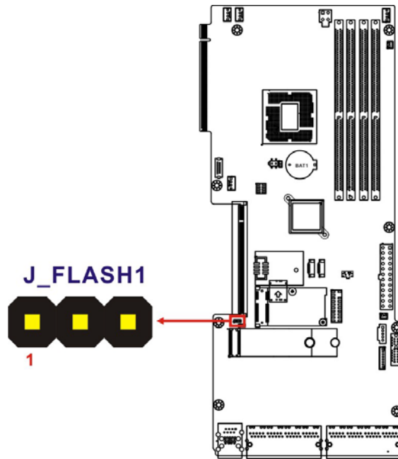
Figure 3-18: Flash Descriptor Security Override Jumper Location
