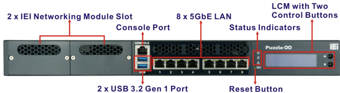
Figure 1-2: PUZZLE-IN001A Front Panel
