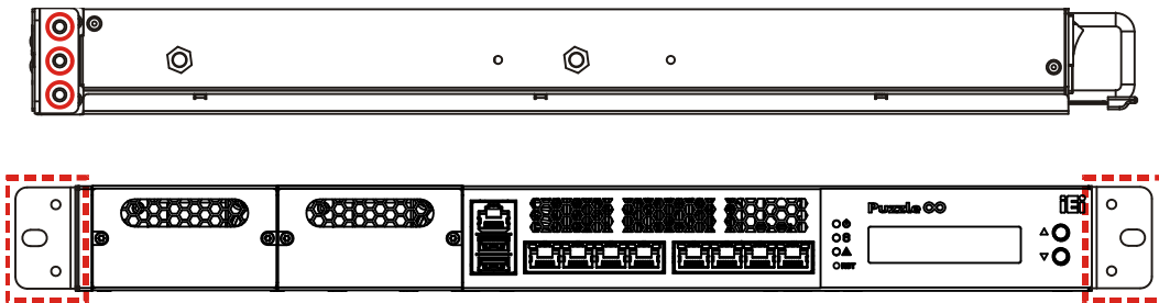
Figure 3-15: Rack Mount Bracket Installation
