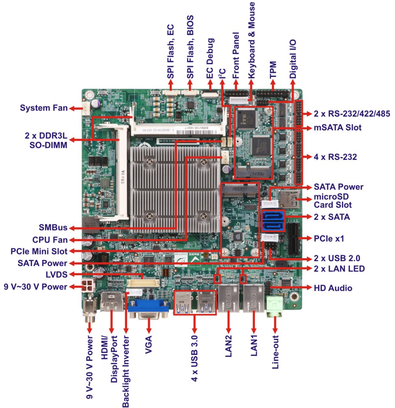
Figure 1-2: Connectors
