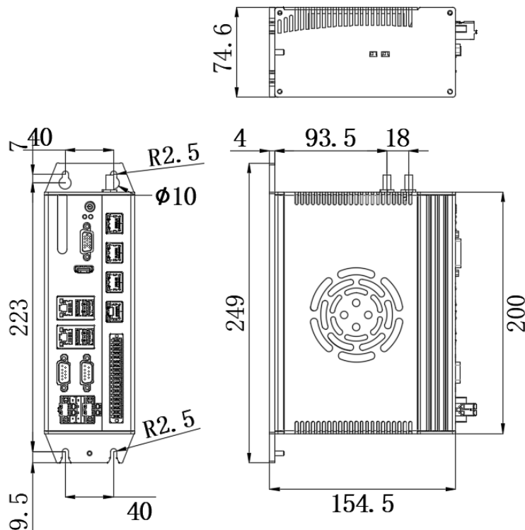
Figure 6 Dimension of NP-6135-H1
