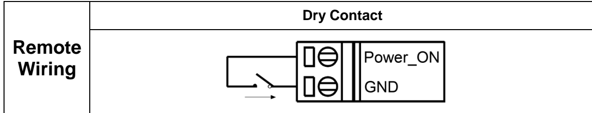
Figure 70 Remote wiring
